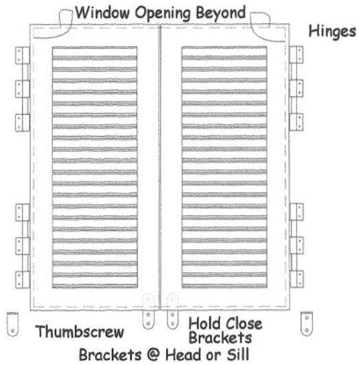
Closed Position
