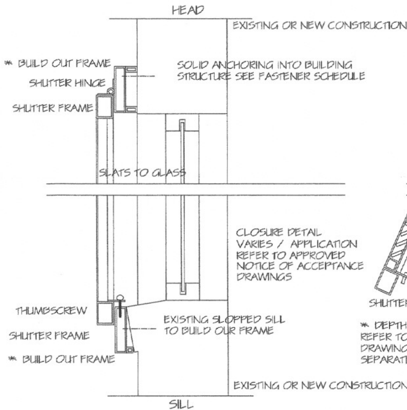
5 HURRICANE BAHAMA or COLONIAL (SIMILAR) SHUTTERS, SILL TO BUILD OUT FRAME BSI EXISTING OR NEW CONSTRUCTION
