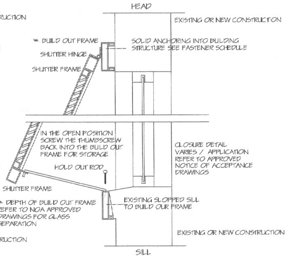
6 HURRICANE BAHAMA SHUTTER OPEN POSITION, SILL TO BUILD OUT FRAME BSI EXISTING OR NEW CONSTRUCTION
