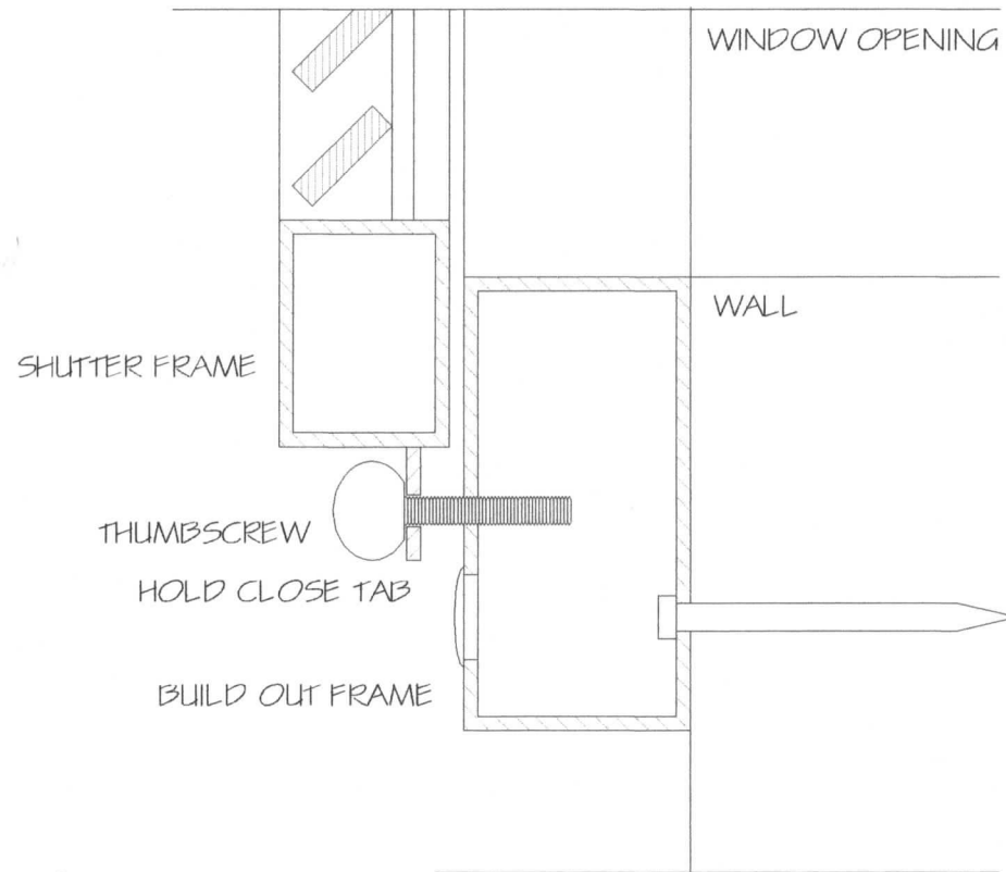
4 HURRICANE SHUTTER OUTSIDE CLOSURE BSI TAB ON SHUTTER WITH THUMBSCREW
