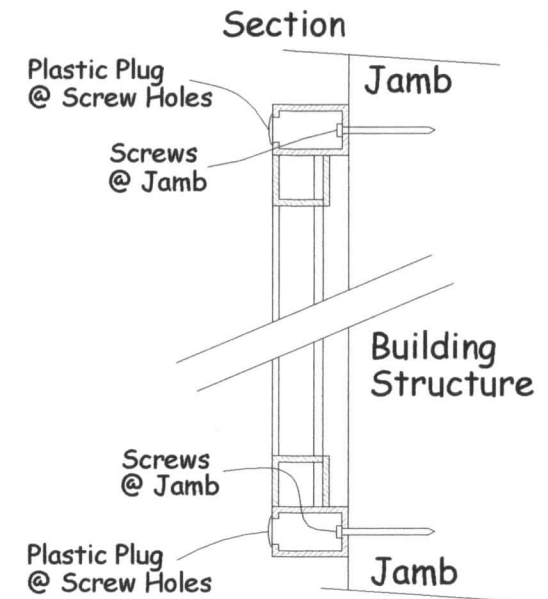
FIGURE 2 - SECTION
