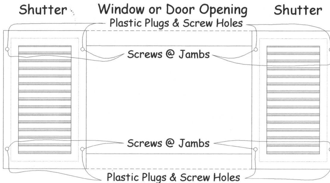
FIGURE 1 - ELEVATION
