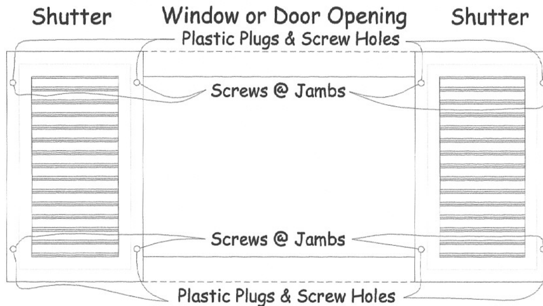
FIGURE 1 - ELEVATION
