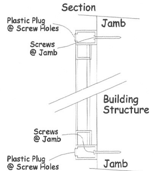
FIGURE 2 - SECTION
