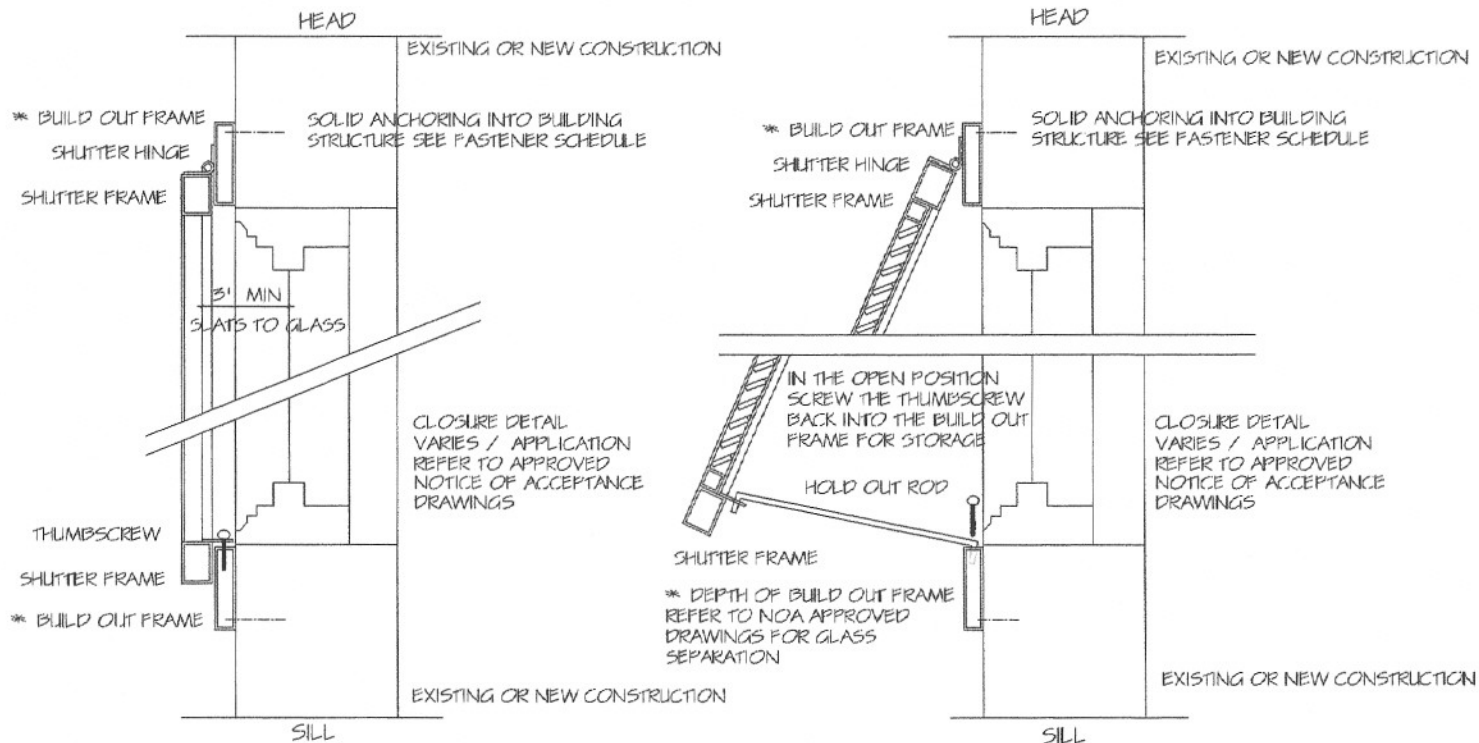
3 HURRICANE BAHAMA SHUTTER CLOSED POSITION BSI EXISTING OR NEW CONSTRUCTION
