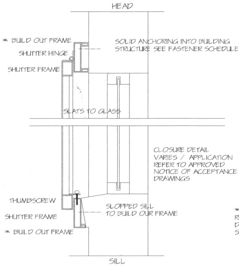
3 HURRICANE BAHAMA CLOSED POSITION BSI BUILD OUT FRAME OVER CONC SILL
