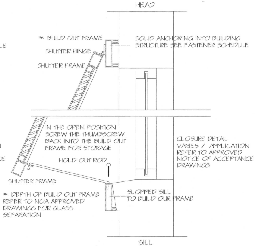
4 HURRICANE BAHAMA OPEN POSITION BSI BUILD OUT FRAME OVER CONC SILL
