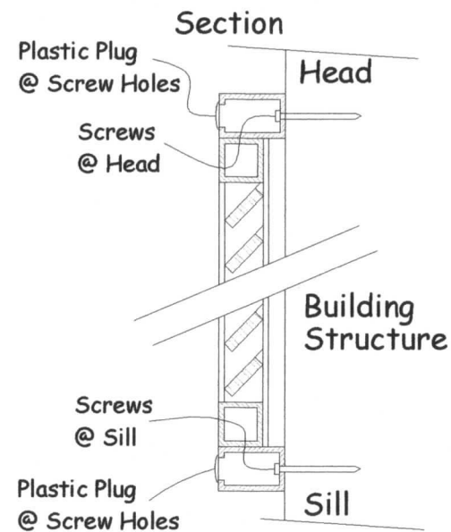
FIGURE 2 - SECTION
