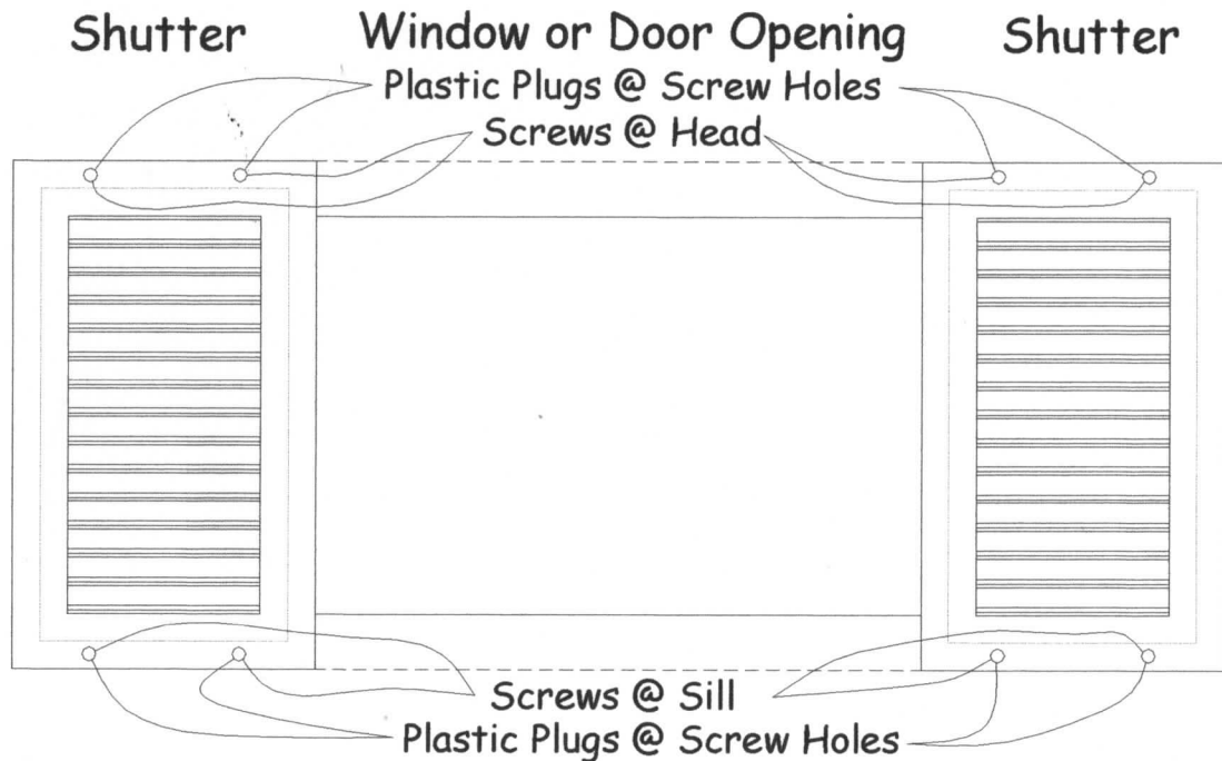
FIGURE 1 - ELEVATION
