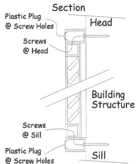
FIGURE 2 - SECTION
