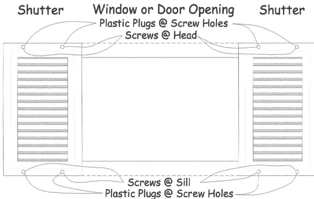
FIGURE 1 - ELEVATION
