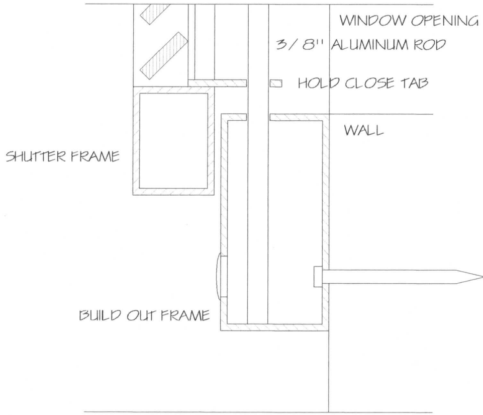
2 HURRICANE SHUTTER, INSIDE CLOSURE BSI WITH ALUMINUM ROD
