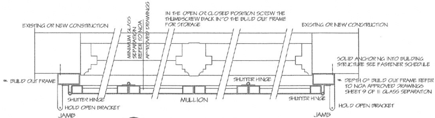
1 HURRICANE COLONIAL SHUTTER CLOSE POSITION BSI EXISTING OR NEW CONSTRUCTION
