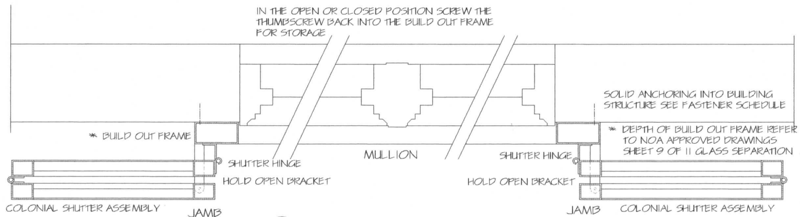
2 HURRICANE COLONIAL SHUTTER BSI OPEN POSITION
