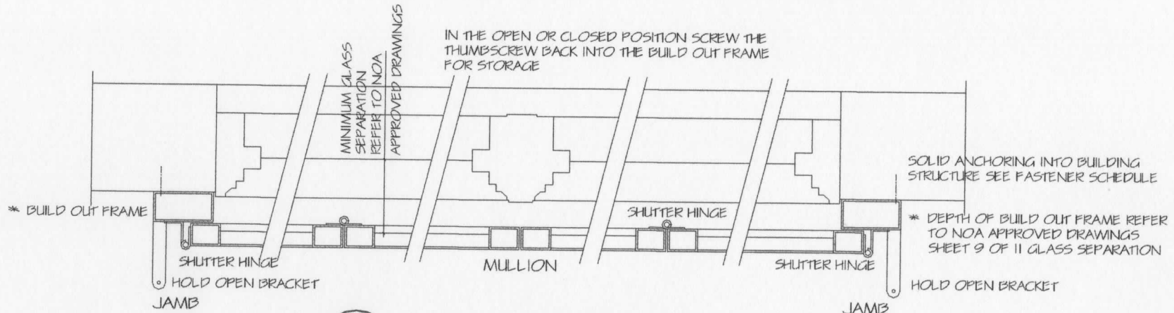
1 HURRICANE COLONIAL SHUTTER BSI CLOSE POSITION
