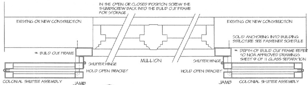
2 HURRICANE COLONIAL SHUTTER OPEN POSITION BSI EXISTING OR NEW CONSTRUCTION
