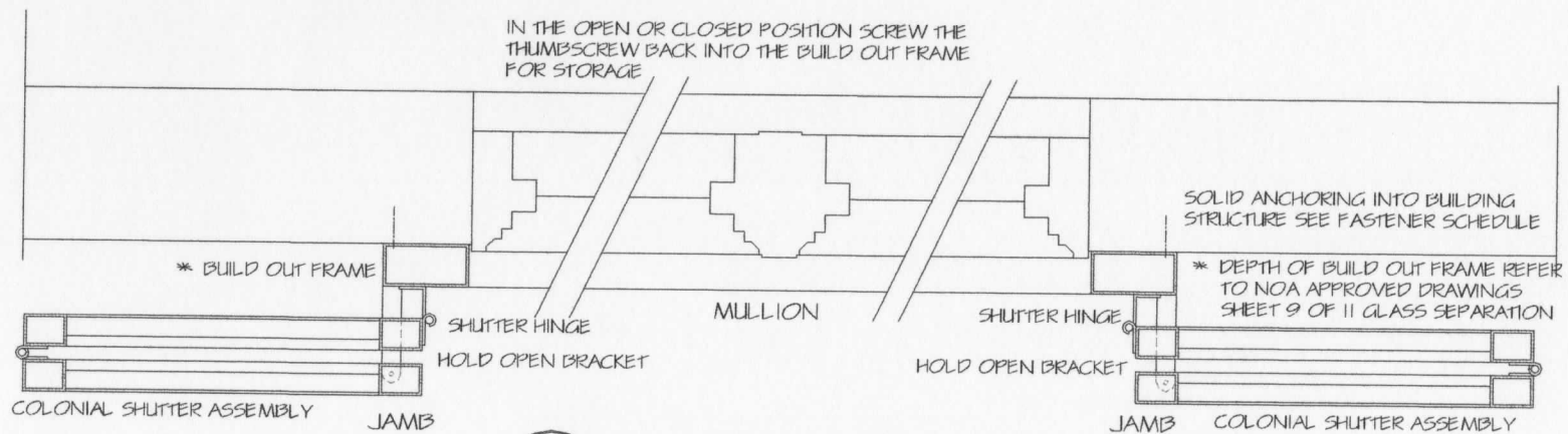
2 HURRICANE COLONIAL SHUTTER BSI OPEN POSITION
