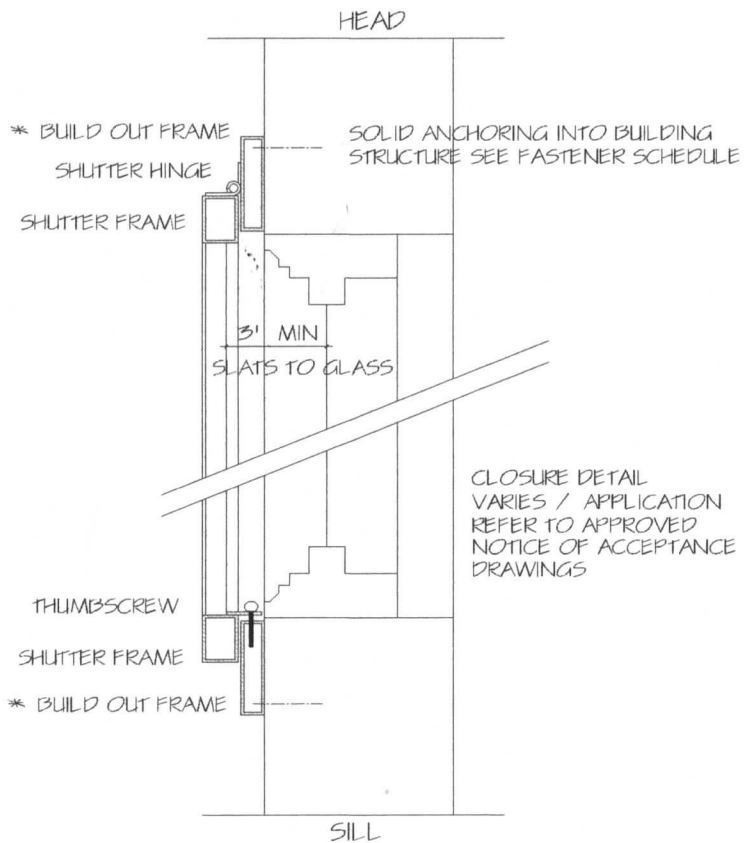
1 HURRICANE BAHAMA SHUTTER BSI CLOSED POSITION
