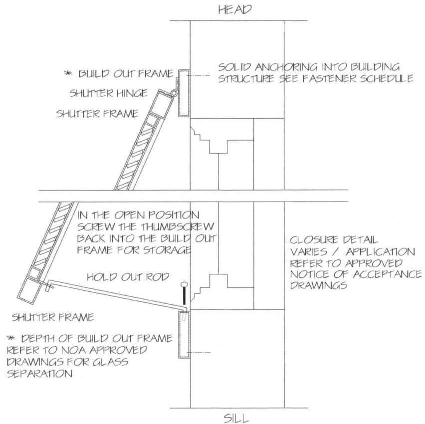
2 HURRICANE BAHAMA SHUTTER BSI OPEN POSITION
