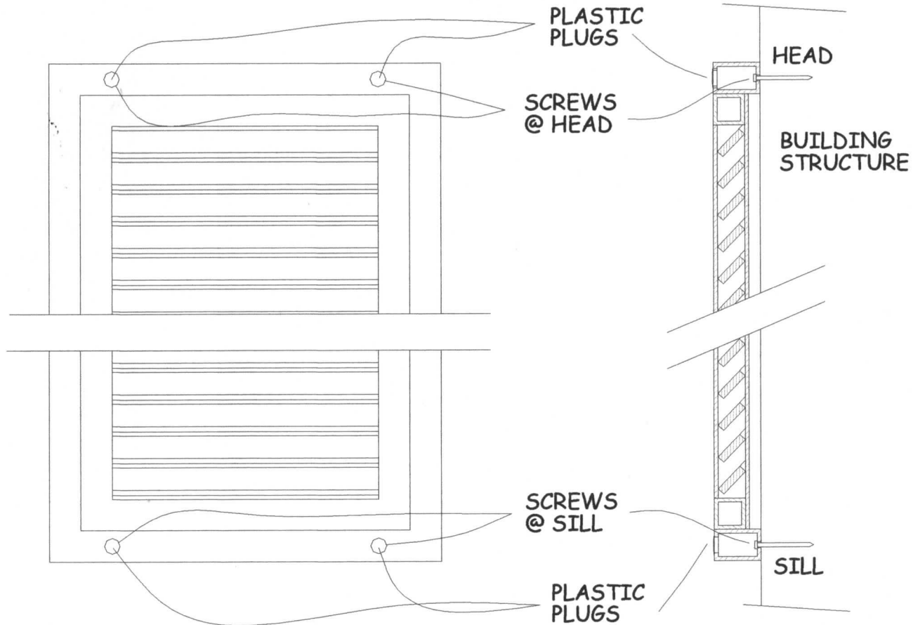
FIGURE 1 - ELEVATION
