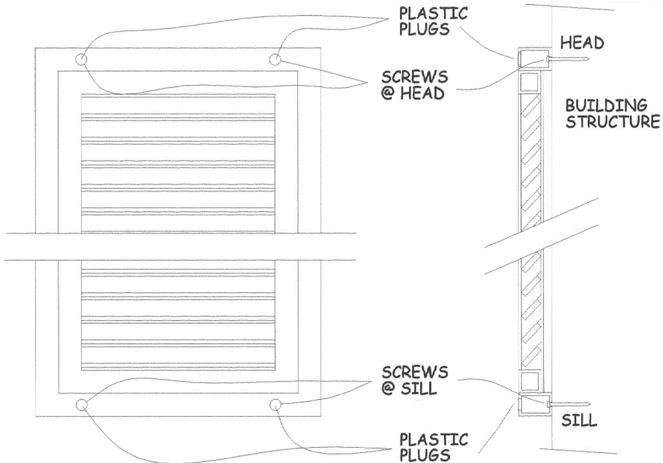
FIGURE 1 - ELEVATION
